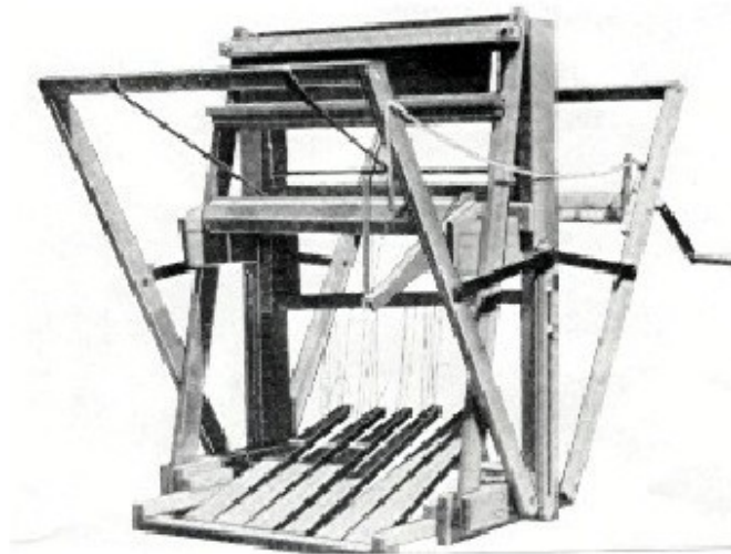
22 Inch Folding Loom
