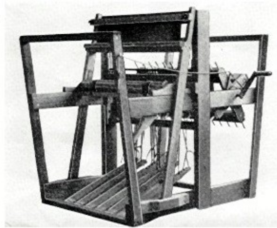
22 Inch Four Harness Loom
